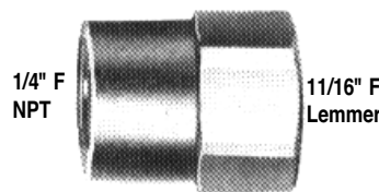
2.10) Gun to Hose adapter; female LEMMER or WAGNER 11/16" gun thread to 1/4" female pipe thread. Made of stainless steel. Order #L033-549. Just add a hose connector which will fit the hose swivel.
