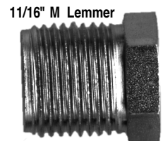
2.3) Tip to Hose adapter; male LEMMER or WAGNER 11/16" gun thread to 3/8" female pipe thread. Order #L033-662. Just add a hose connector which will fit the hose swivel.
