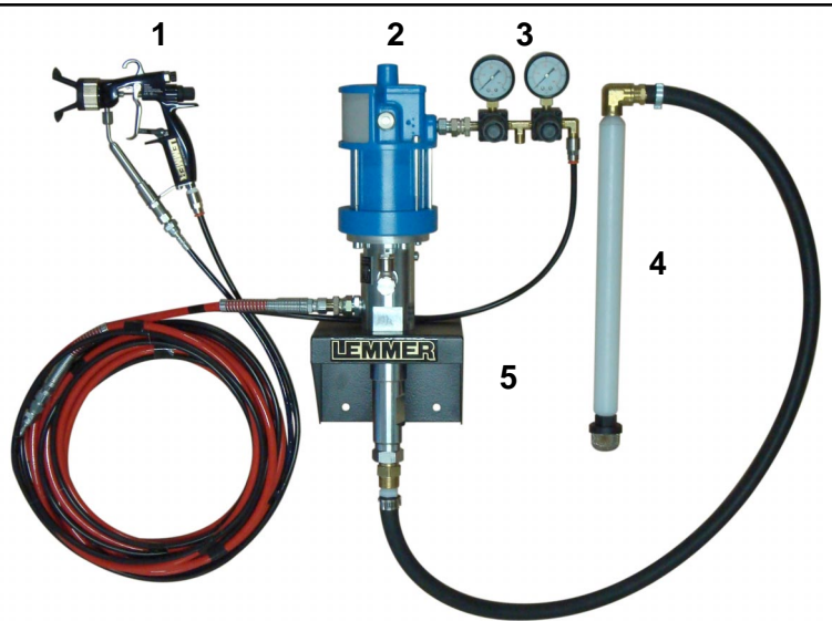
3033 wall-mount system, order number ....L011-038
